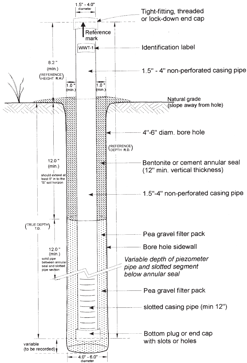
Figure 1. CROSS SECTION OF TYPICAL GROUNDWATER PIEZOMETER
