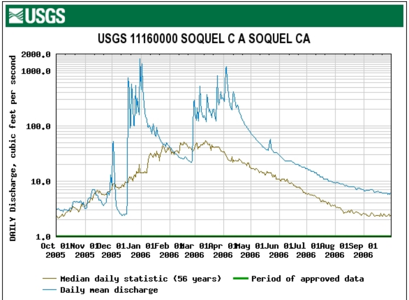
Figure 31. The 2006 Daily Mean and Median Flow at the USGS Gage on Soquel Creek at Soquel.
