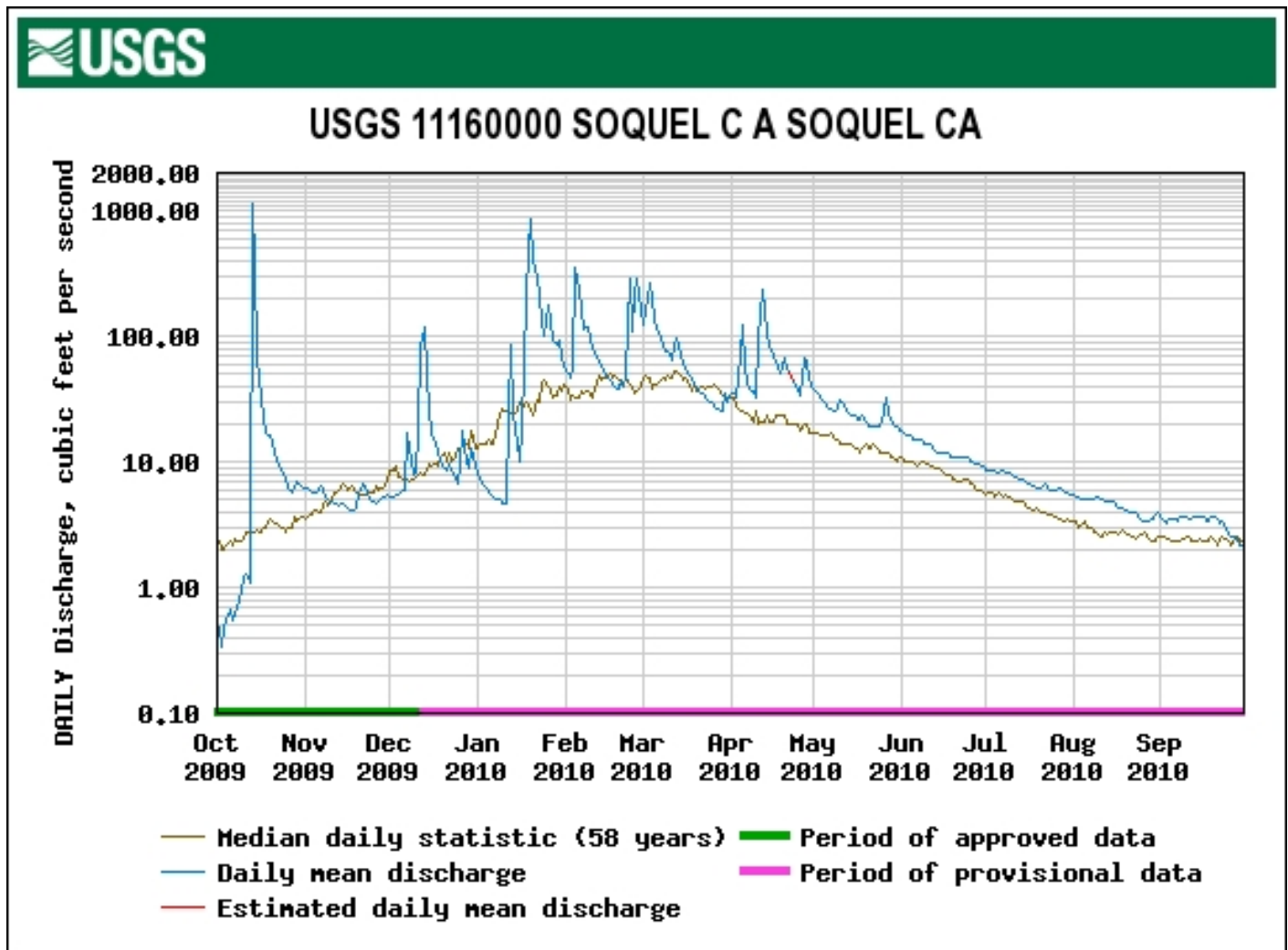
Figure 35. The 2010 Daily Mean and Median Flow at the USGS Gage on Soquel Creek at Soquel.
