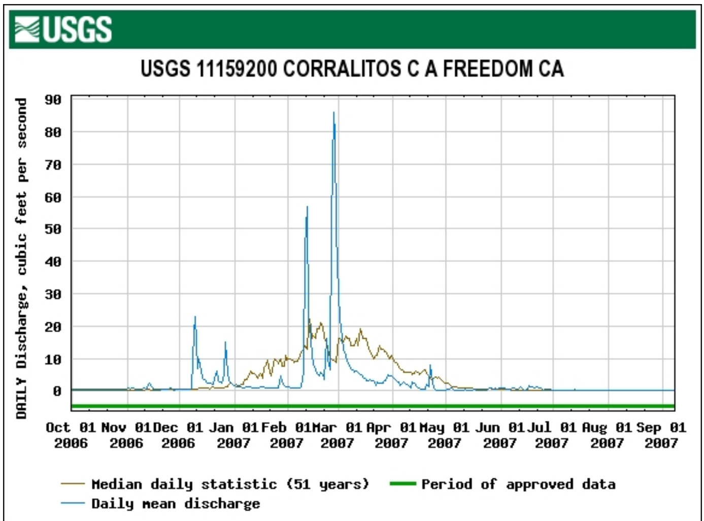
Figure 42. The 2007 Daily Mean and Median Flow at the USGS Gage on Corralitos Creek at Freedom. (USGS website would not provide a logarithmic scale of discharge).
