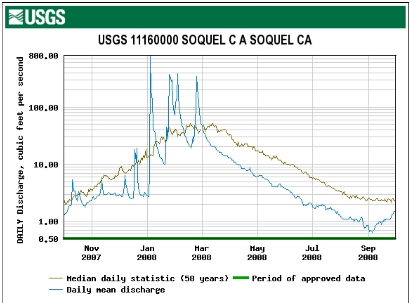
Figure 33. The 2008 Daily Mean and Median Flow at the USGS Gage on Soquel Creek at Soquel.
