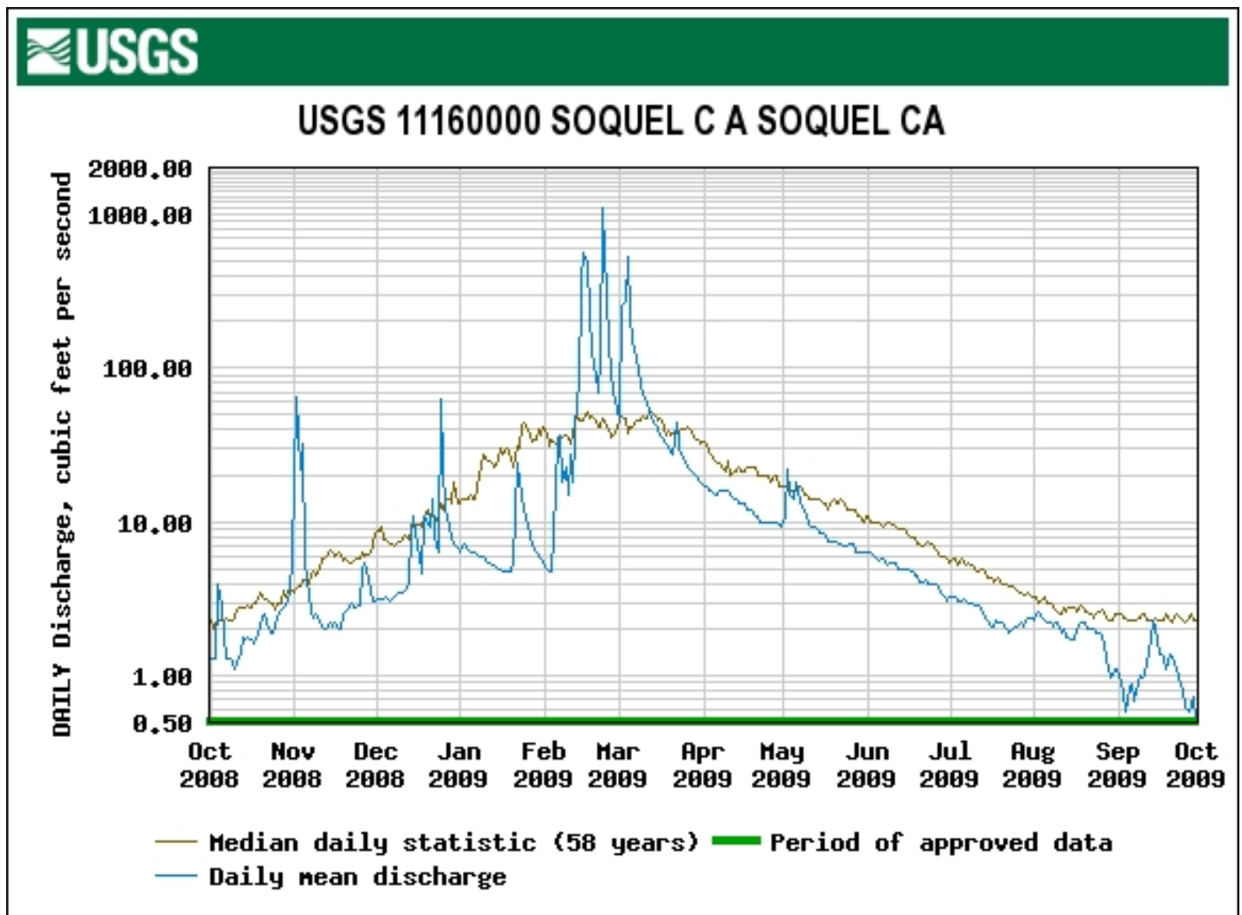
Figure 34. The 2009 Daily Mean and Median Flow at the USGS Gage on Soquel Creek at Soquel.
