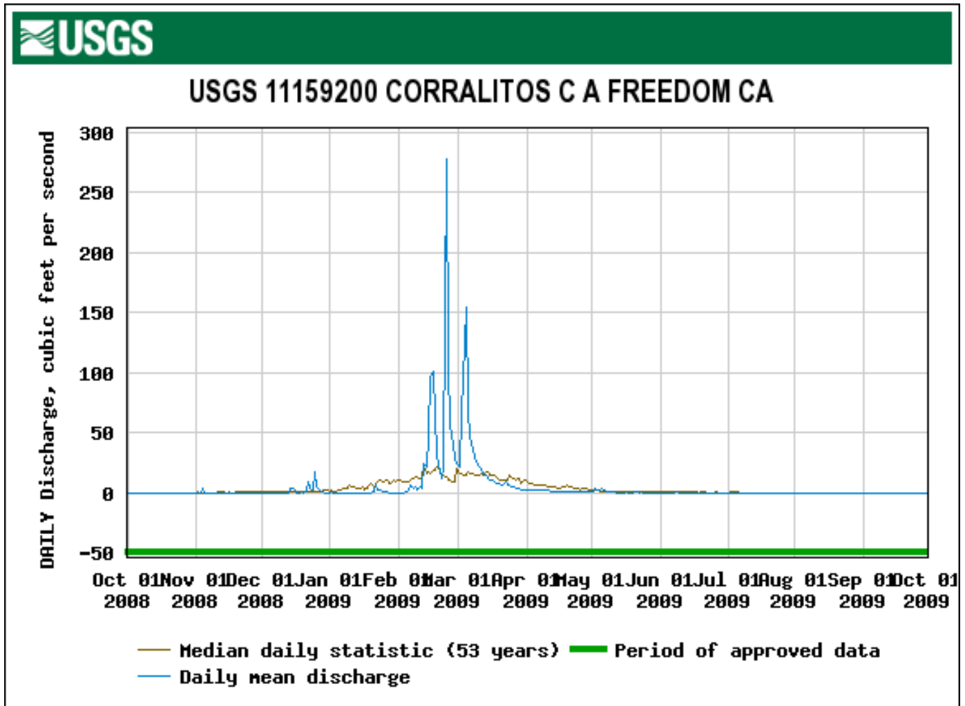
Figure 44. The 2009 Daily Mean and Median Flow at the USGS Gage on Corralitos Creek at Freedom. (USGS website would not provide a logarithmic scale of discharge).
