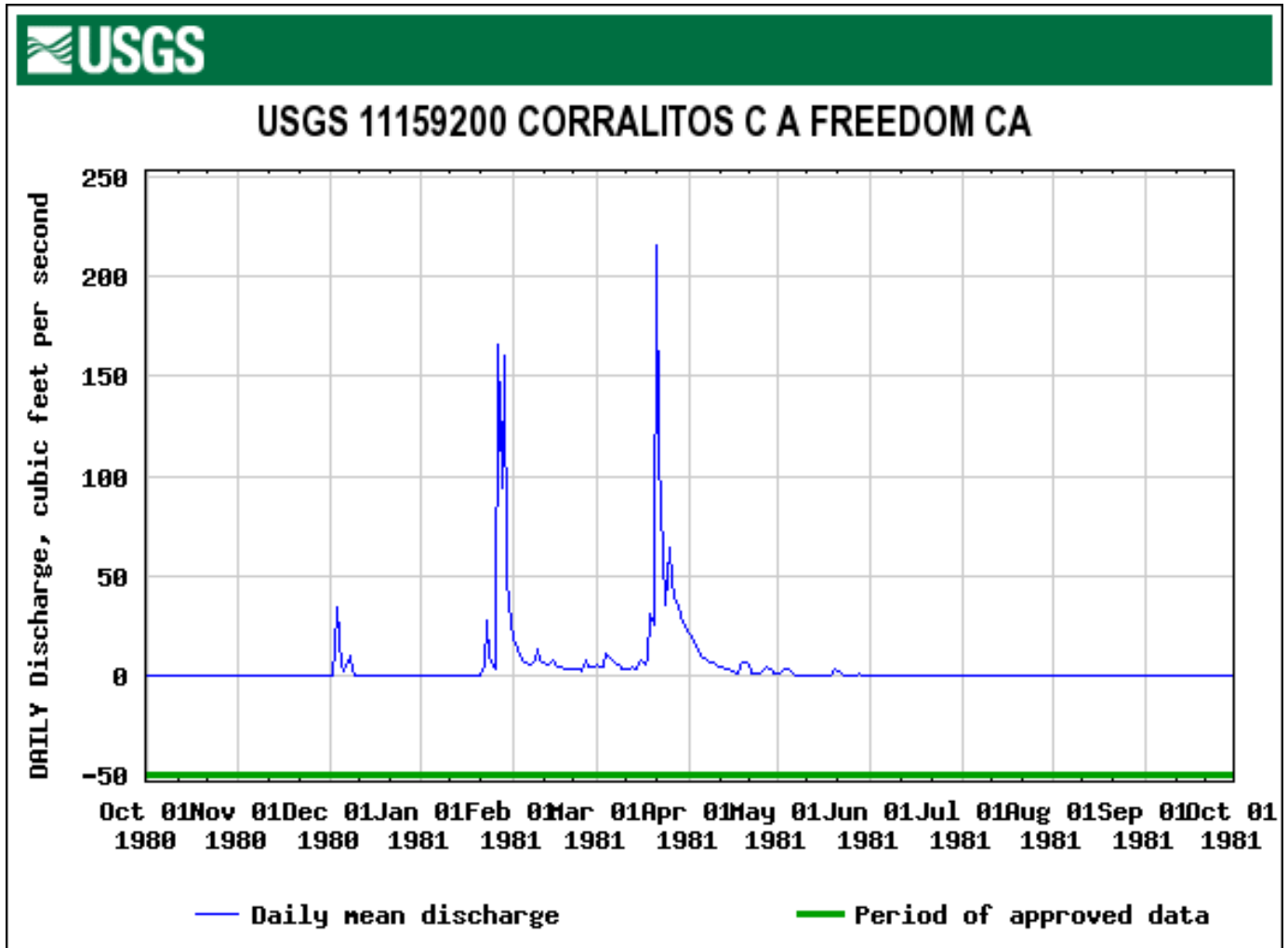
Figure 38. The 1981 Daily Mean Flow at the USGS Gage on Corralitos Creek at Freedom. (USGS website would not provide logarithmic scale of discharge.)
