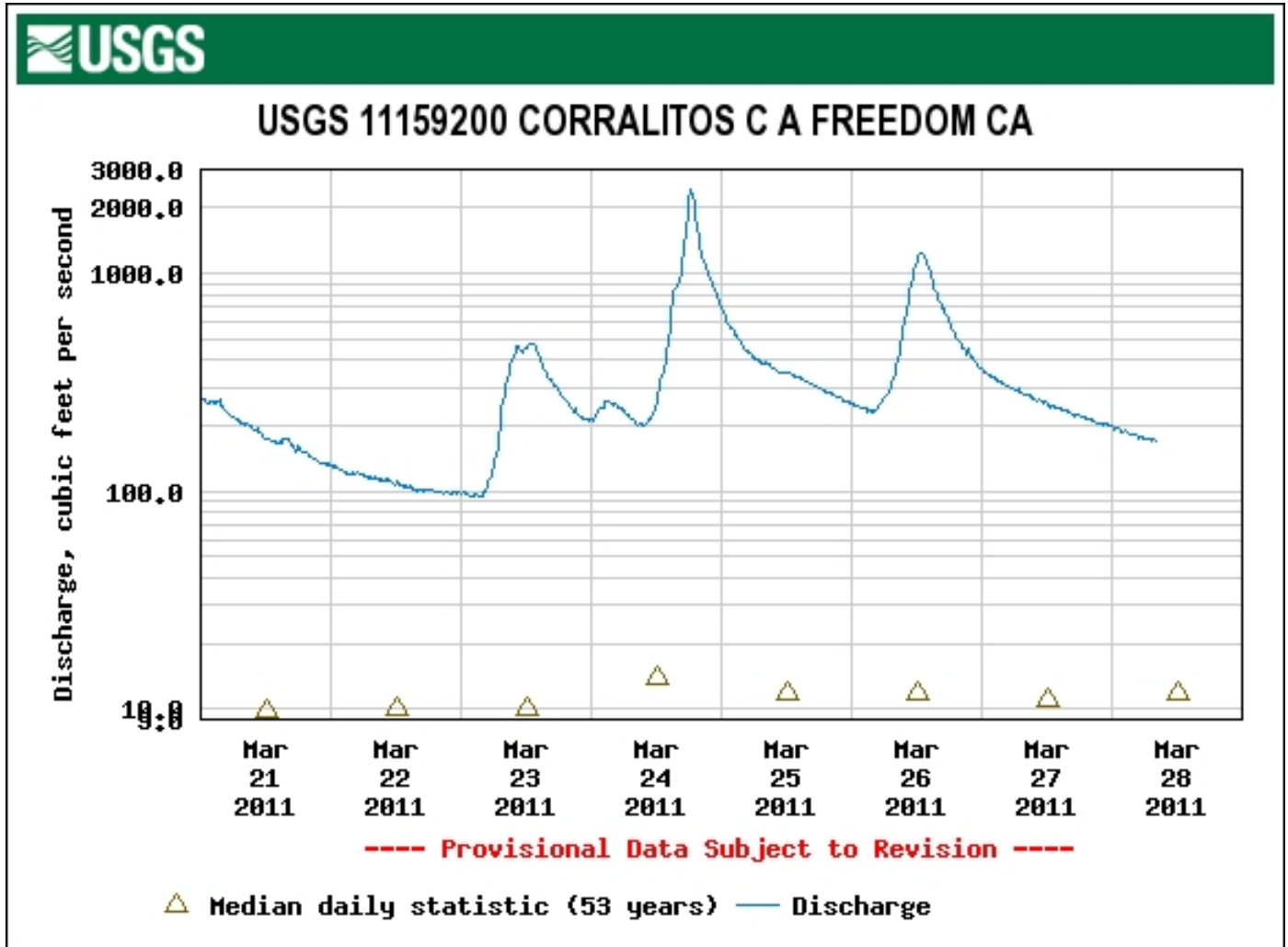
Figure 47. The Late March 2011 Discharge of Record for the USGS Gage on Corralitos Creek at Freedom.
