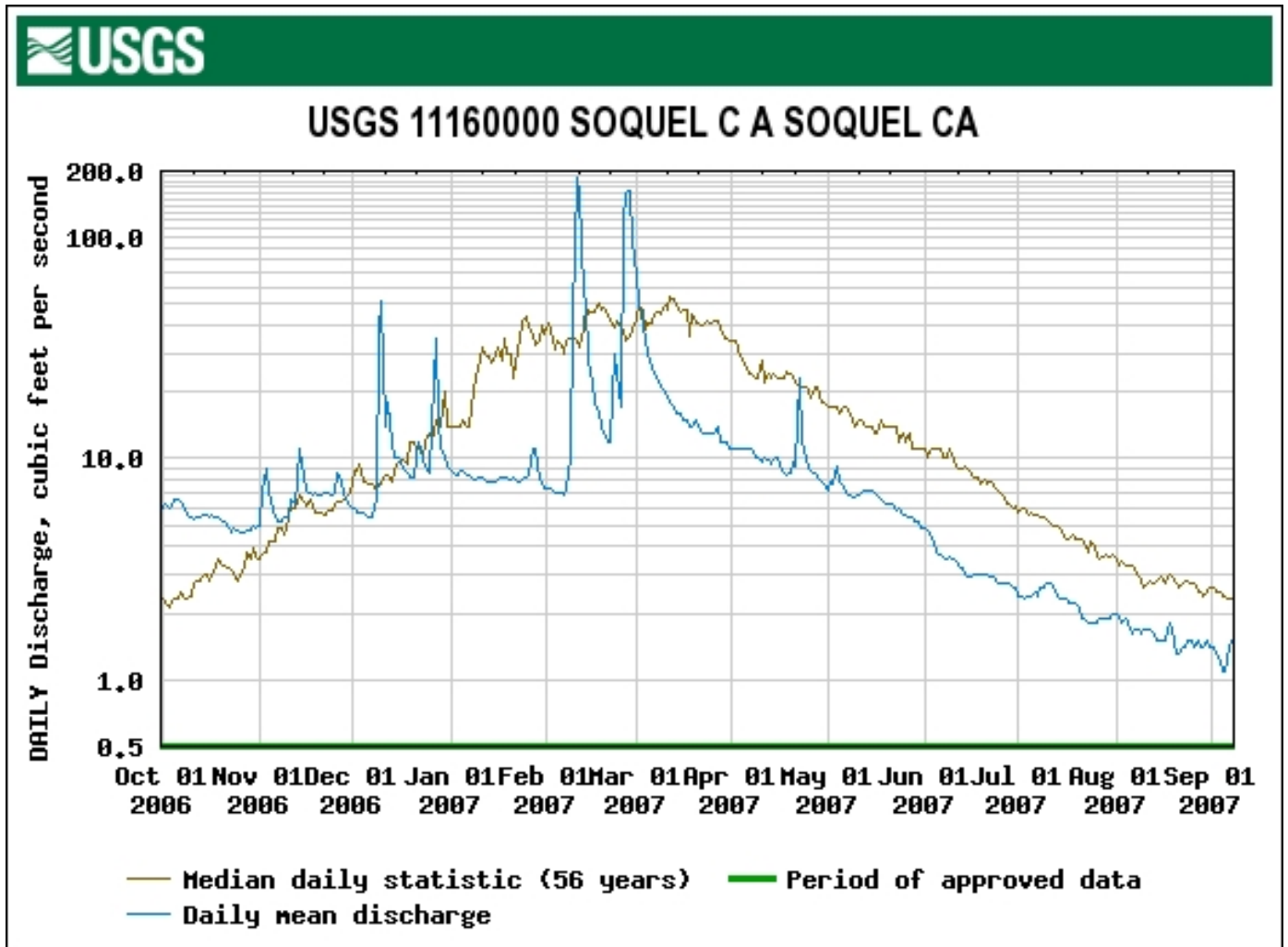
Figure 32. The 2007 Daily Mean and Median Flow at the USGS Gage on Soquel Creek at Soquel.
