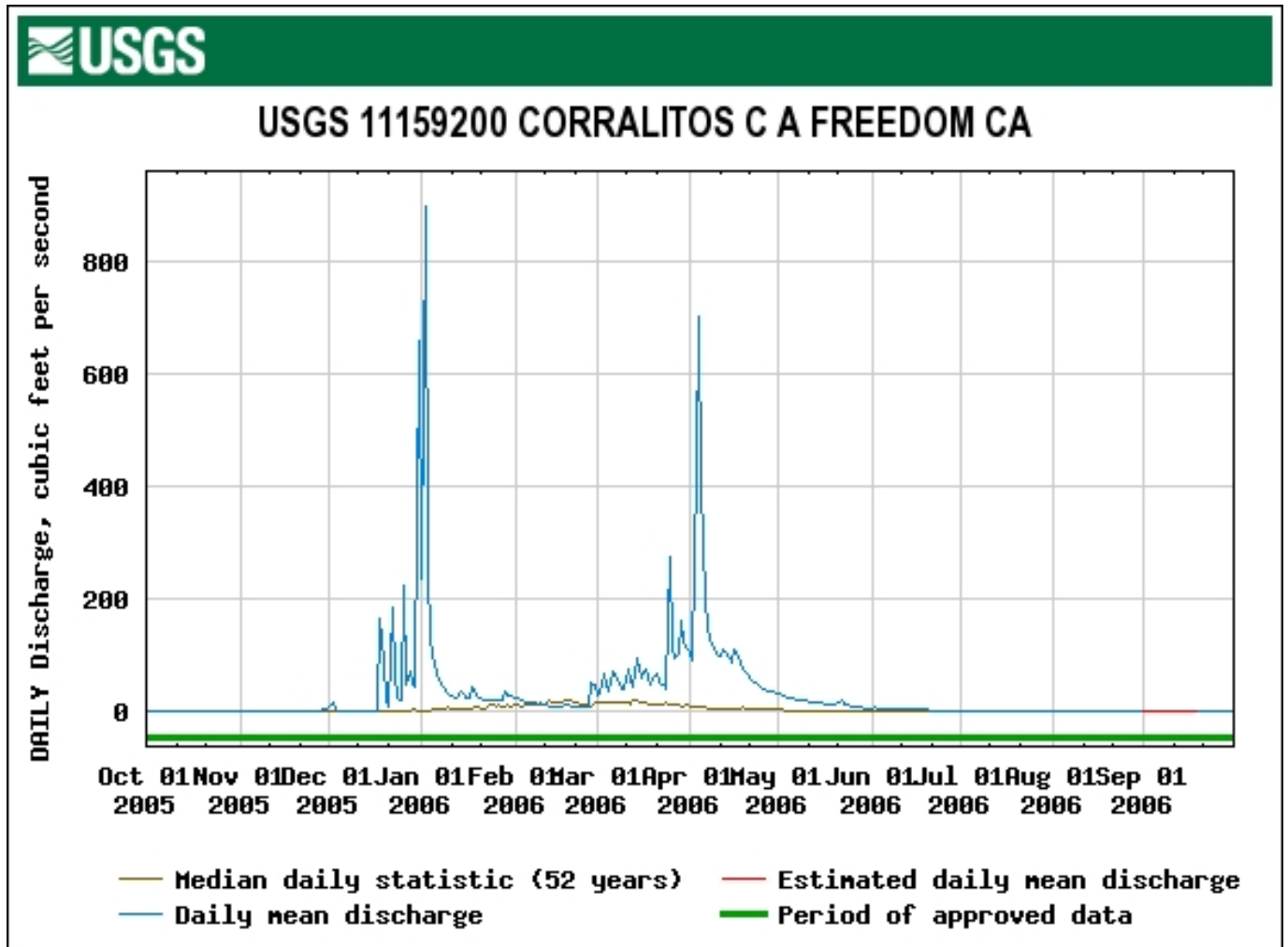
Figure 41. The 2006 Daily Mean Flow at the USGS Gage on Corralitos Creek at Freedom with Median Flow Statistics.
