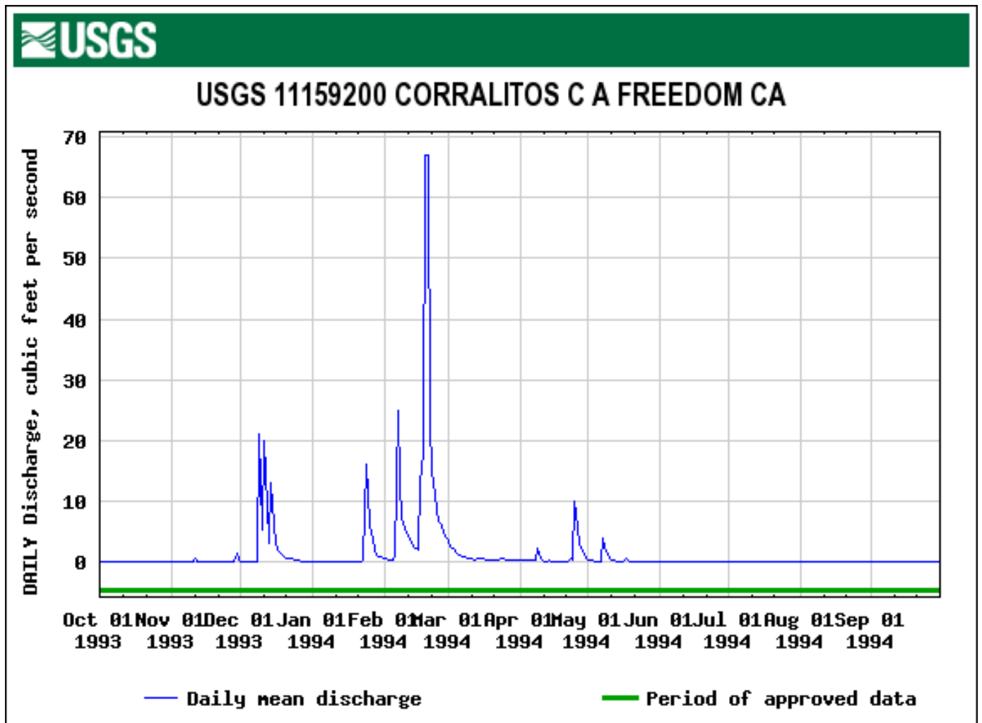
Figure 39. The 1994 Daily Mean Flow at the USGS Gage on Corralitos Creek at Freedom. (USGS website would not provide logarithmic scale of discharge.)
