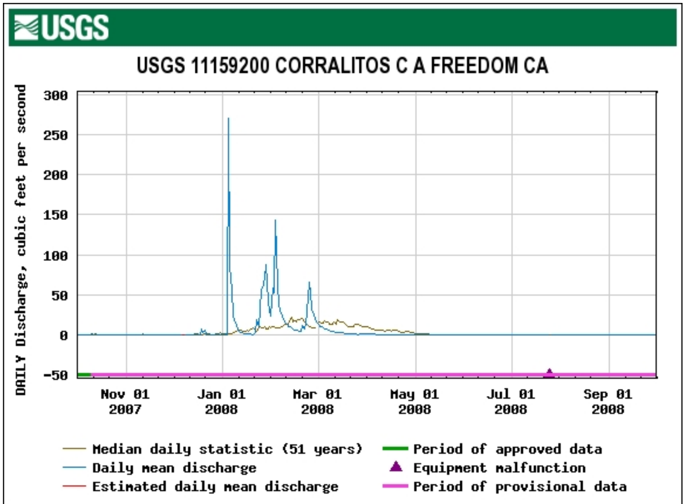
Figure 43. The 2008 Daily Mean and Median Flow at the USGS Gage on Corralitos Creek at Freedom. (USGS website would not provide a logarithmic scale of discharge).
