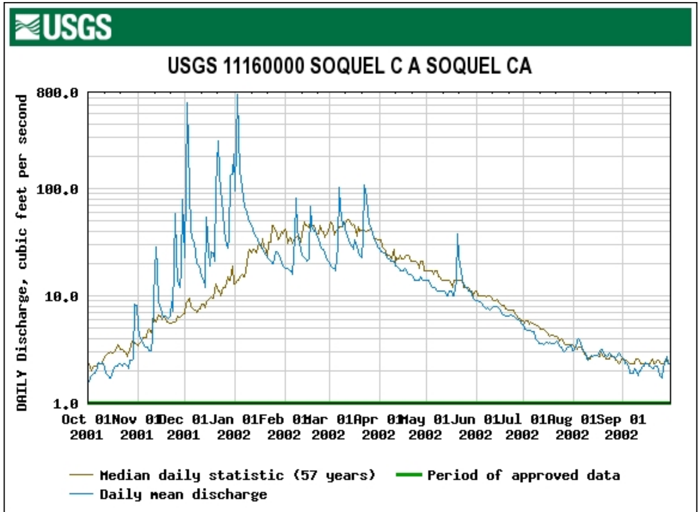
Figure 27. The 2002 Daily Mean and Peak Flood Flow at the USGS Gage on Soquel Creek at Soquel.
