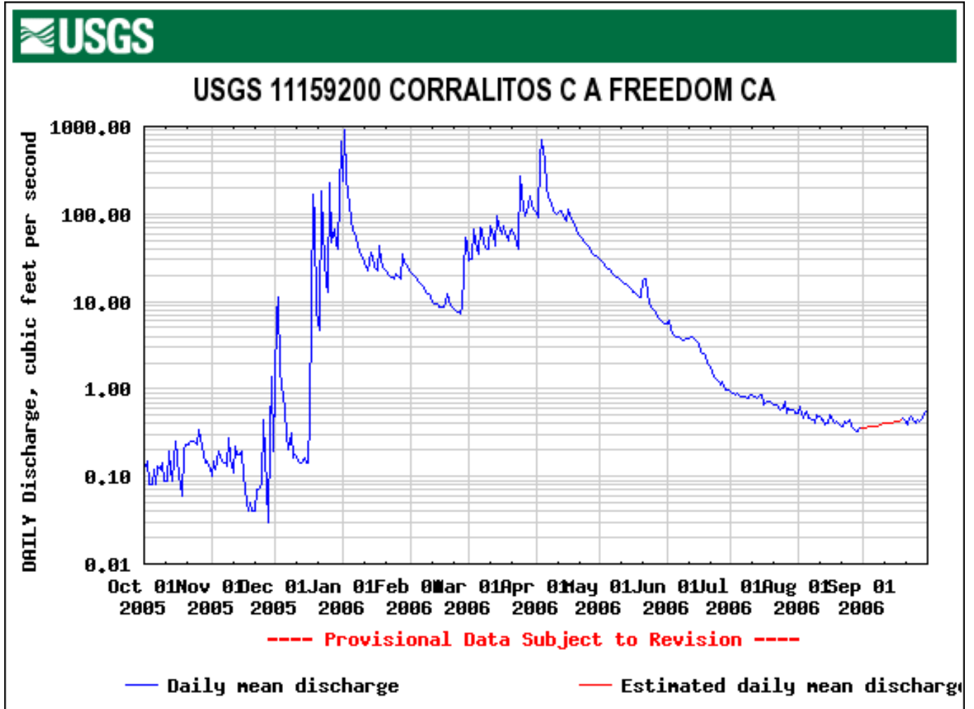
Figure 40. The 2006 Daily Mean Flow at the USGS Gage on Corralitos Creek at Freedom.
