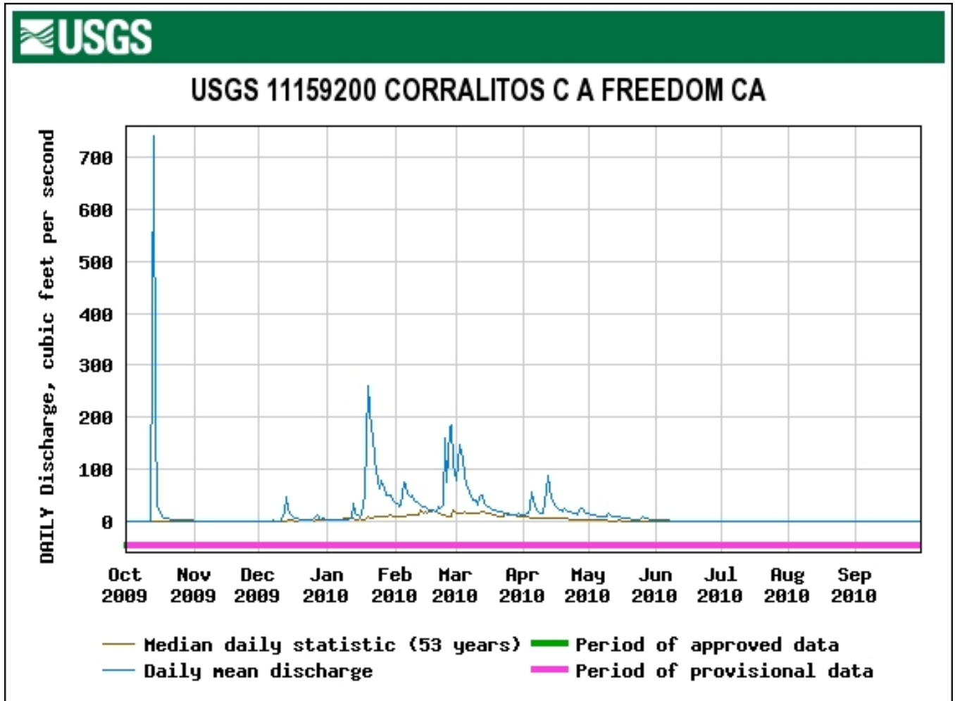
Figure 45. The 2010 Daily Mean and Median Flow at the USGS Gage on Corralitos Creek at Freedom. (USGS website would not provide a logarithmic scale of discharge).
